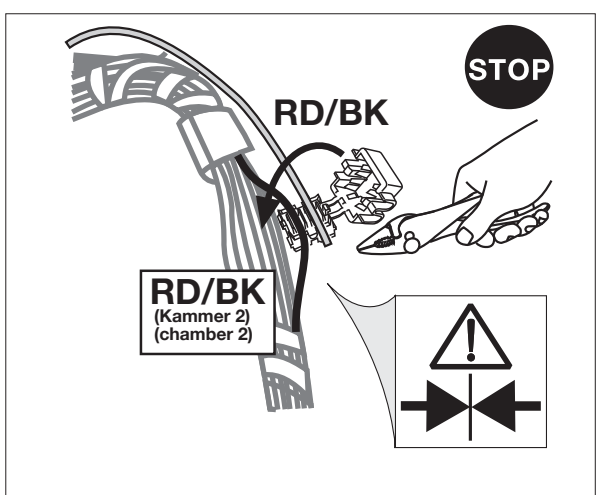
Steckhülsegehäuse 32-polig (GY) Connector 32-pin (GY)
