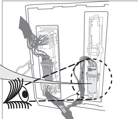
Steckhülsegehäuse 32-polig (GY) Connector 32-pin (GY)
